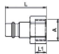
Plug female
