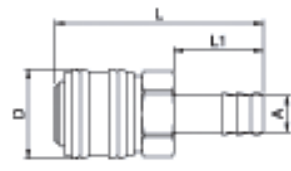
Hose connection
